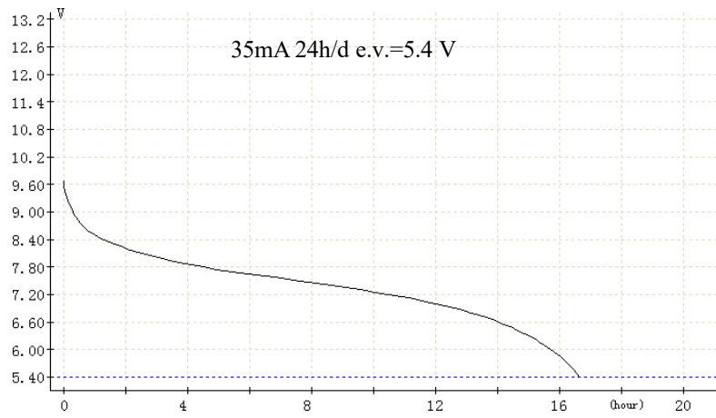
Chart 1. Discharge diagram
