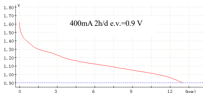
Chart 1. Discharge diagram
